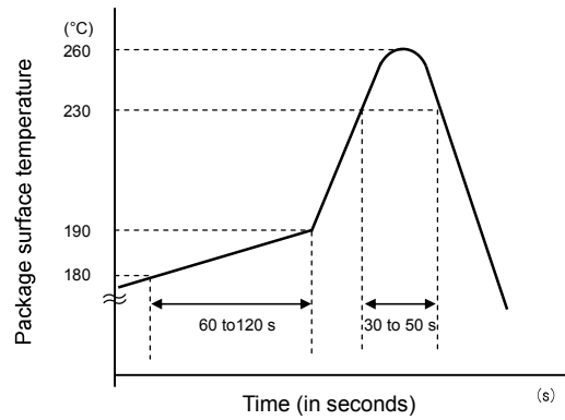
Figure 2 Example of Temperature Profile
