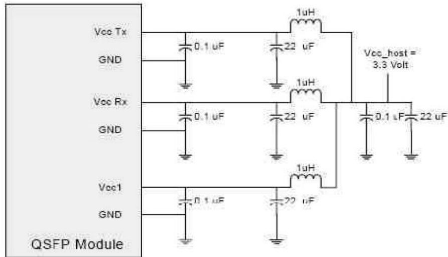
QSFPP Host Recommended Circuit
