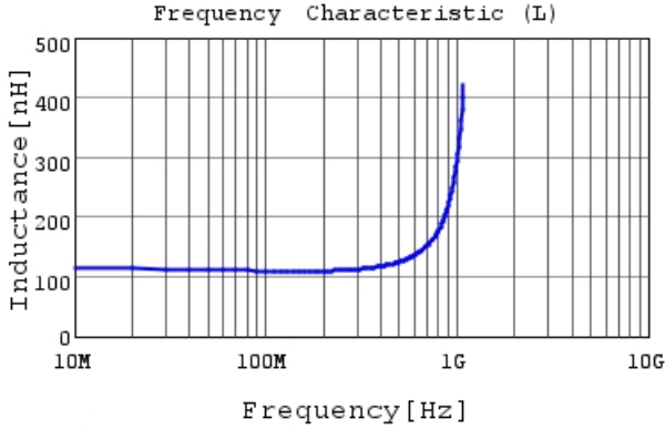
LQG15WHR11G02 L
