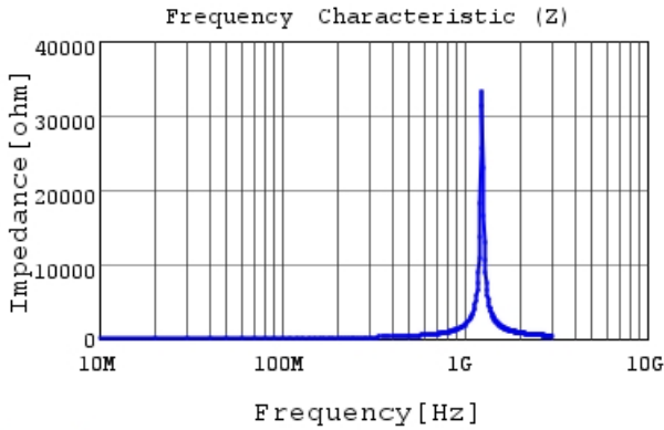
LQG15WHR11G02 |Z|
