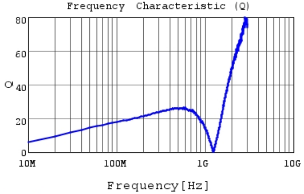
LQG15WHR11G02 Q
