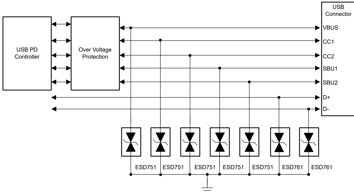
Typical Application
