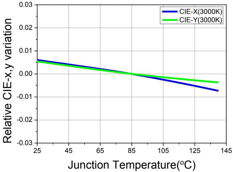
Fig 10. Junction Temperature vs. CIE x,y Shift, I_f=0.54A (CRI80, 3000K)
