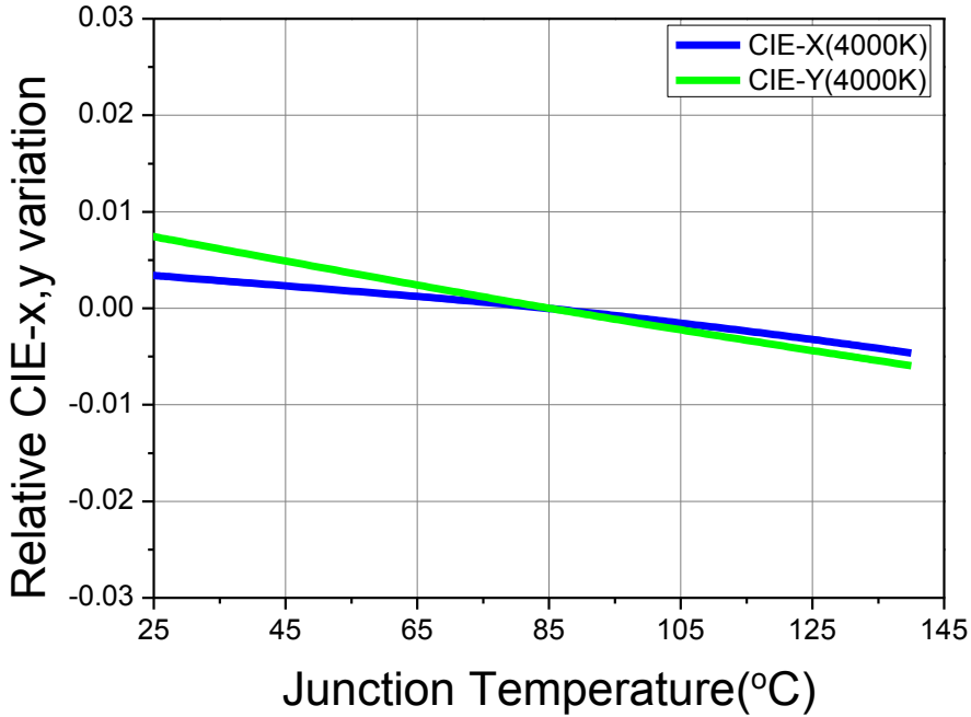
Fig 11. Junction Temperature vs. CIE x,y Shift, I_f=0.54A (CRI90, 4000K)
