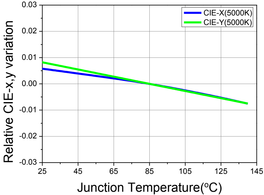
Fig 8. Junction Temperature vs. CIE x,y Shift, I_F=0.54A (CRI80, 5000K)
