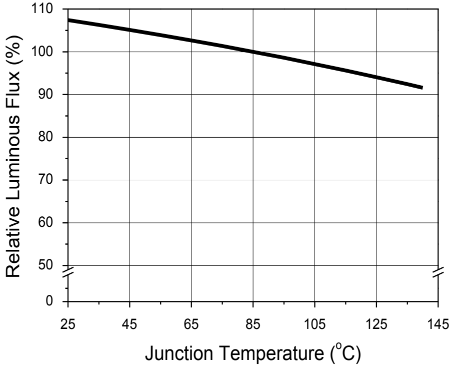
Fig 6. Junction Temperature vs. Relative Luminous Flux, I_F=0.54A
