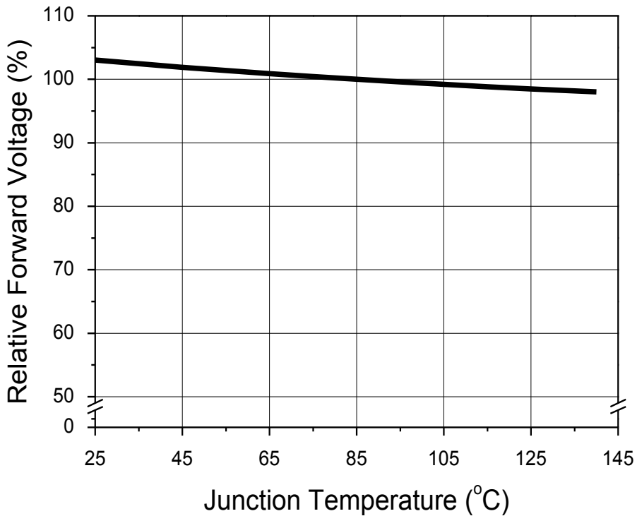
Fig 7. Junction Temperature vs. Forward Voltage, I_F=0.54A
