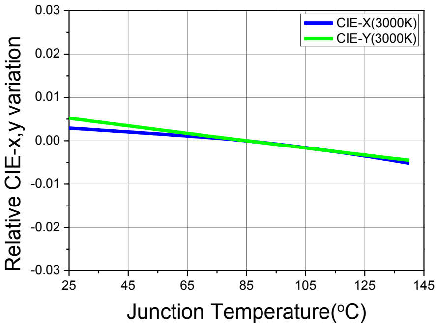
Fig 12. Junction Temperature vs. CIE x,y Shift, I_f=0.54A (CRI90, 3000K)
