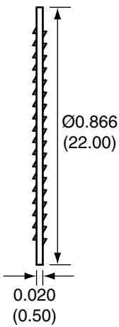
WASHER
