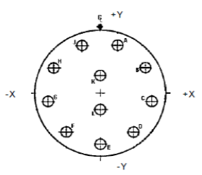
Contact Layout
