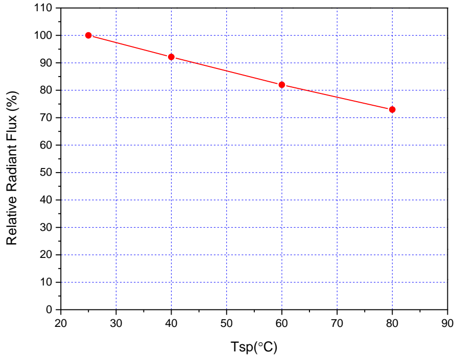
Fig 5. Relative Optical Output Power vs. Solder Point Temperature, I_F=20mA
