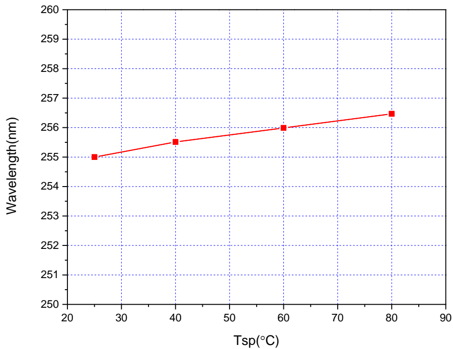
Fig 6. Peak Wavelength vs. Solder Point Temperature, I_F=20mA
