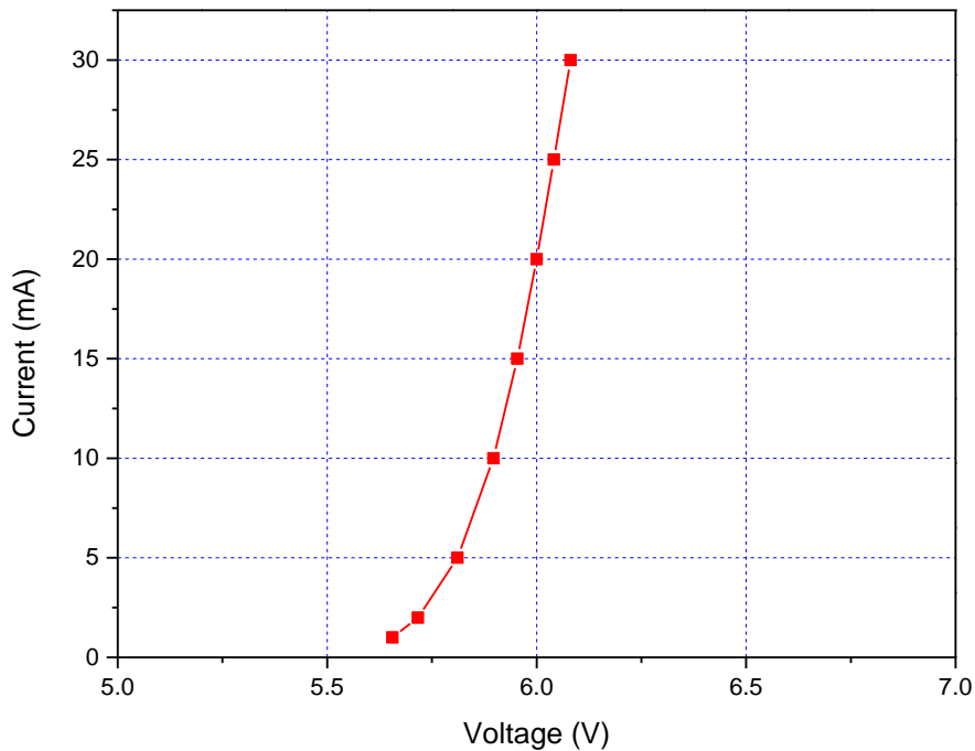
Fig 2. Forward Current vs Forward Voltage, T_a=25^\circ\text{C}
