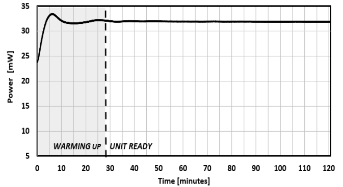
FIG. 4: WARM-UP TIME
