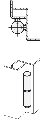
Installation example
