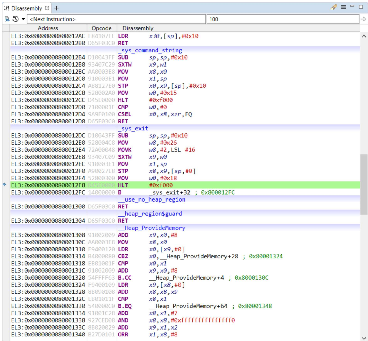
Figure 9-14: Disassembly view
