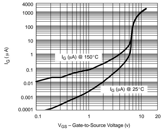
Gate-Source Voltage vs. Gate-Current
