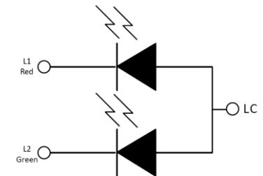
LED Schematic
