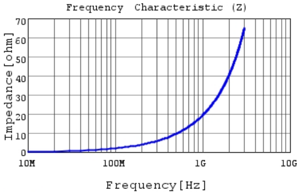
LQG15WH3N1C02 |Z|
