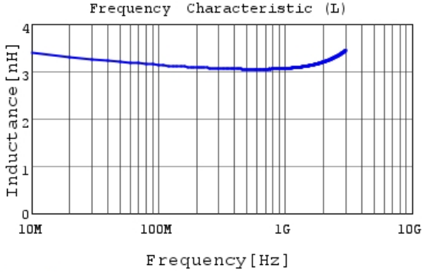
LQG15WH3N1C02 L
