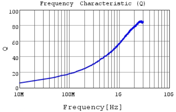
LQG15WH3N1C02 Q
