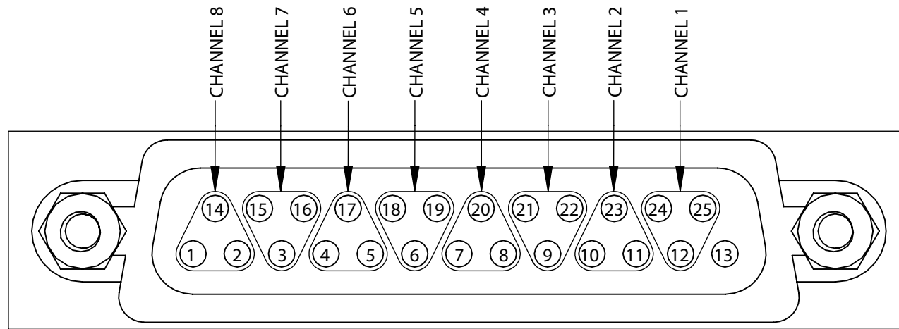
DB25 CONNECTOR PINOUT
