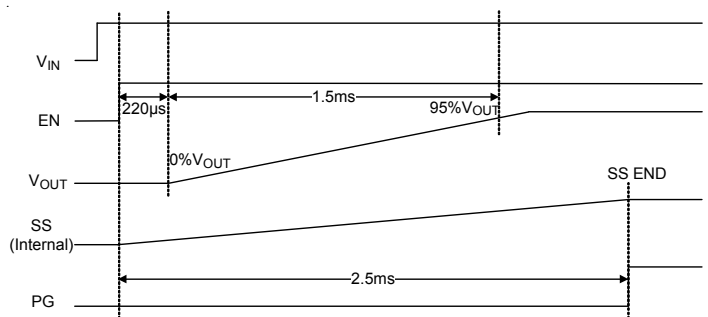
Figure 1. Start-Up Sequence
