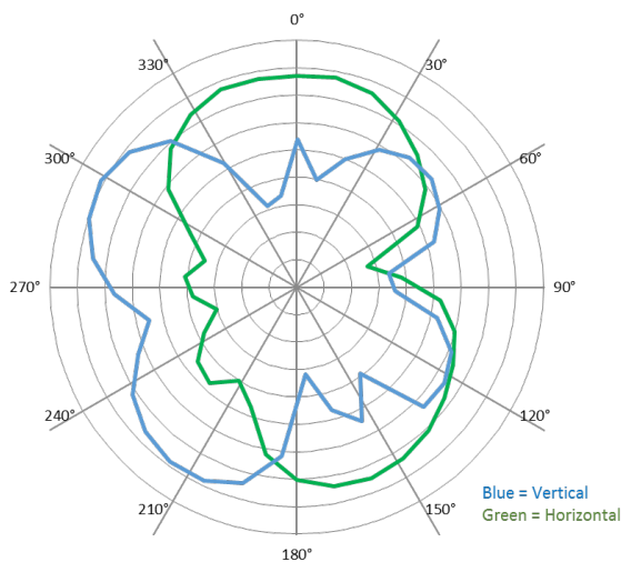
Figure 9: X-Y plane antenna pattern
