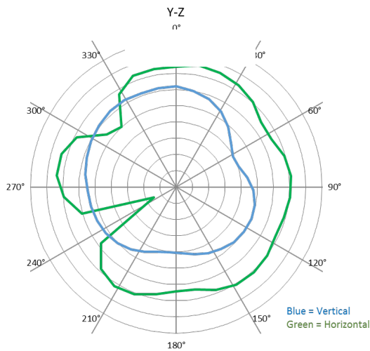
Figure 11: Y-Z plane antenna pattern
