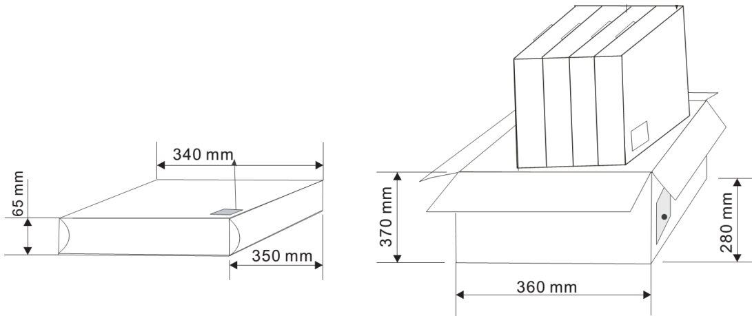
Figure 12: Reel cartons used for type number BMD-330-A-R-00
