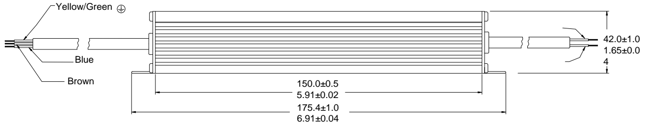
Side View
