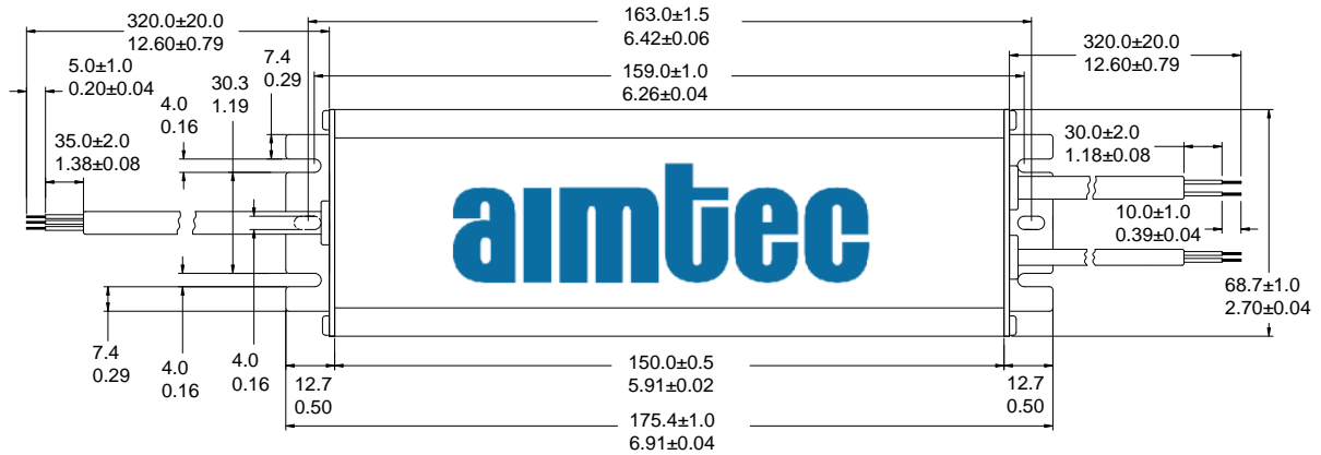
Side View
