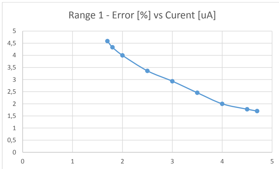
Figure 2.8-1.1.8 50kΩ Sinking
