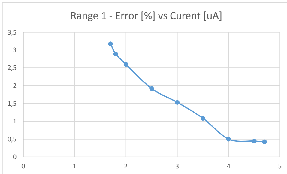
Figure 2.8.1.4 50kΩ Sourcing
