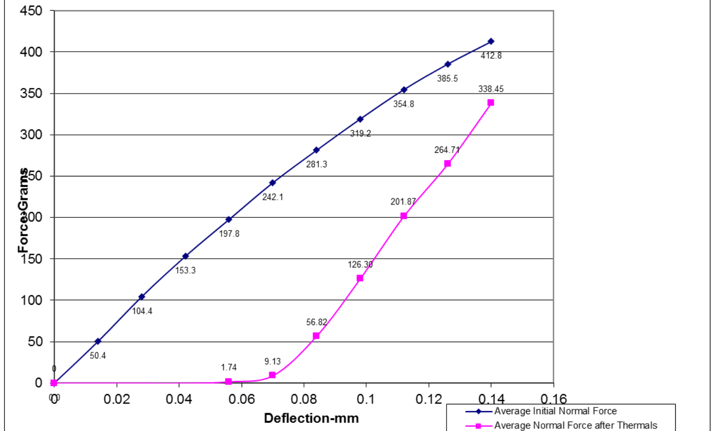
Normal Force - Average Initial vs Average Thermal
