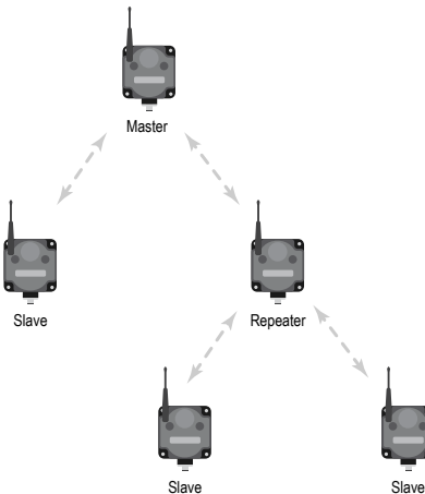
Figure 5. Tree network
