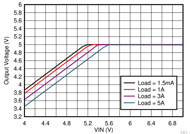
V_{OUT} = 5\text{ V} f_{SW} = 2200\text{ kHz} FPWM Mode
