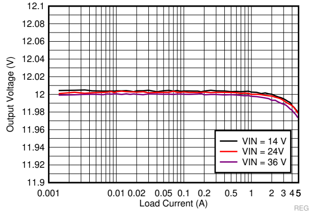
V_{OUT} = 12\text{ V} f_{SW} = 500\text{ kHz} FPWM Mode
