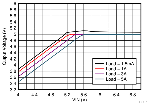
V_{OUT} = 5\text{ V} f_{SW} = 2200\text{ kHz} Auto Mode
