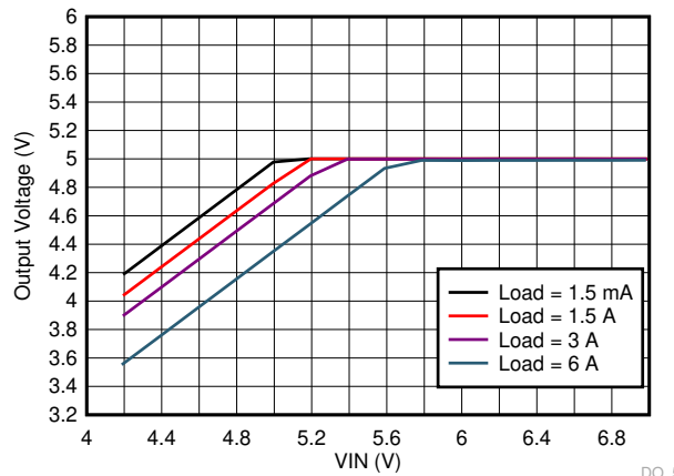
V_{OUT} = 5\text{ V} f_{SW} = 400\text{ kHz} FPWM Mode
