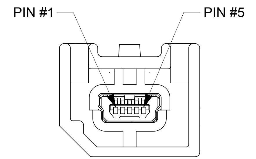
MATING HEADER FOR MINI-B PLUGS (POLARIZATION - A SHOWN)
