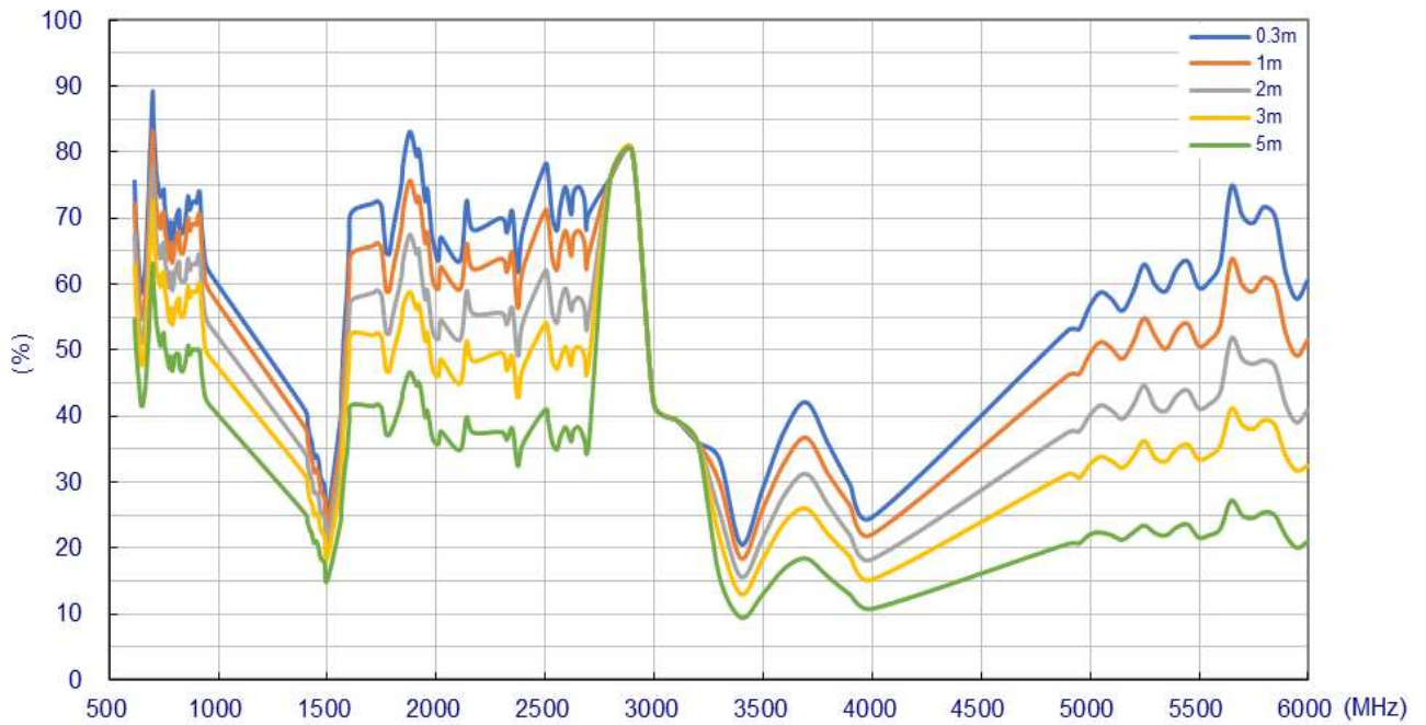
Figure 10. Efficiency of GSA.8842 Antenna with different cable lengths
