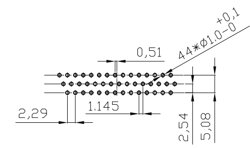
44 Pin Female Connector PCB Pin Layout
