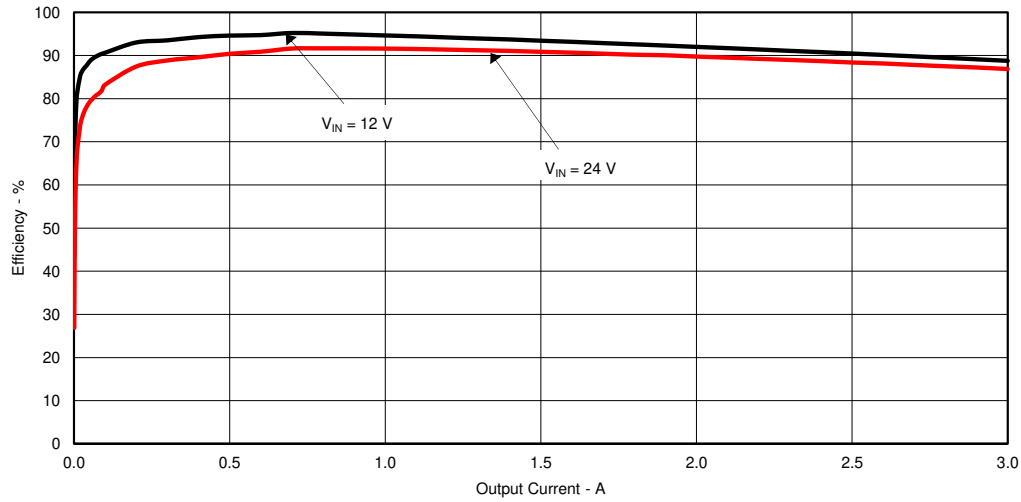
Figure 2-1. TPS54335AEVM-010 Efficiency
