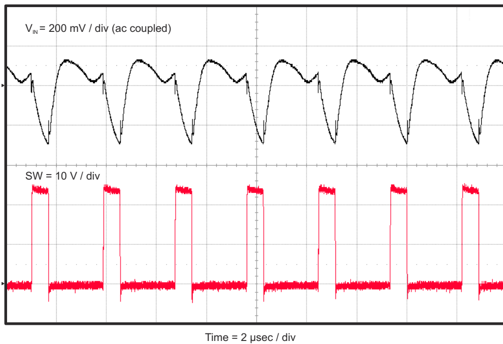
Figure 2-10. TPS54335AEVM-010 Input Ripple
