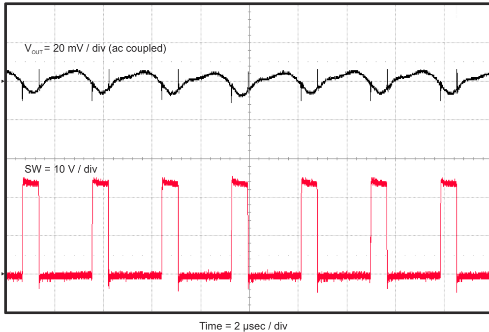
Figure 2-7. TPS54335AEVM-010 Output Ripple, I_{OUT} = 3\text{ A}
