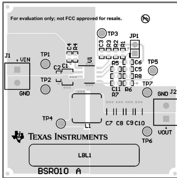
Figure 3-2. TPS54335AEVM-010 Top-Side Layout
