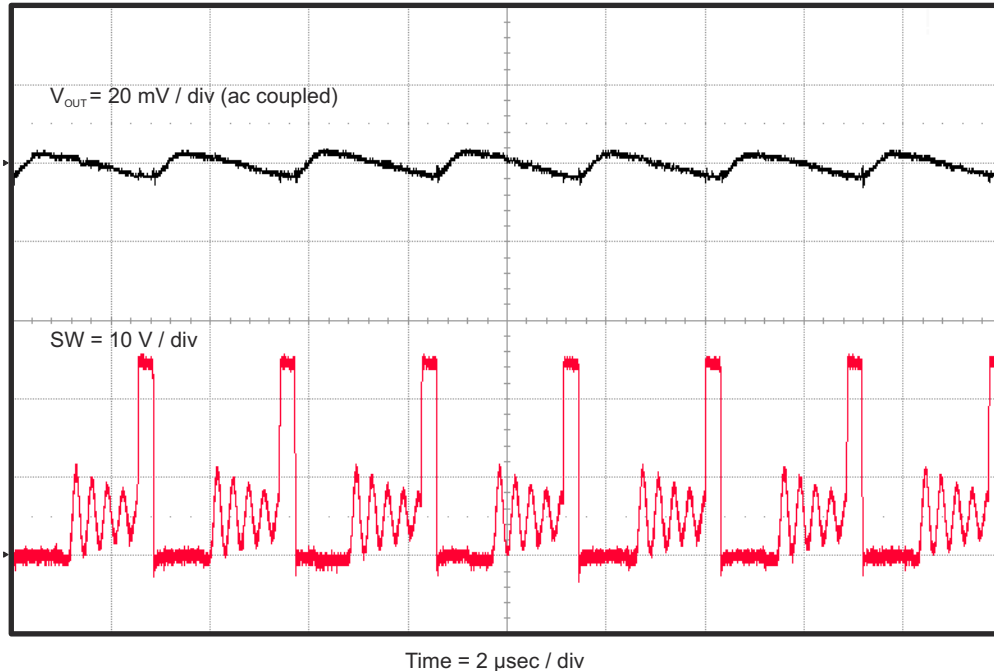
Figure 2-8. TPS54335AEVM-010 Output Ripple, I_{OUT} = 100\text{ mA}
