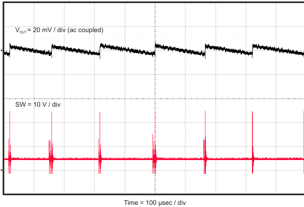
Figure 2-9. TPS54335AEVM-010 Output Ripple, I_{OUT} = 0 \text{ A}
