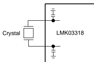
Figure 36. Crystal Reference Input Configuration During Device Test
