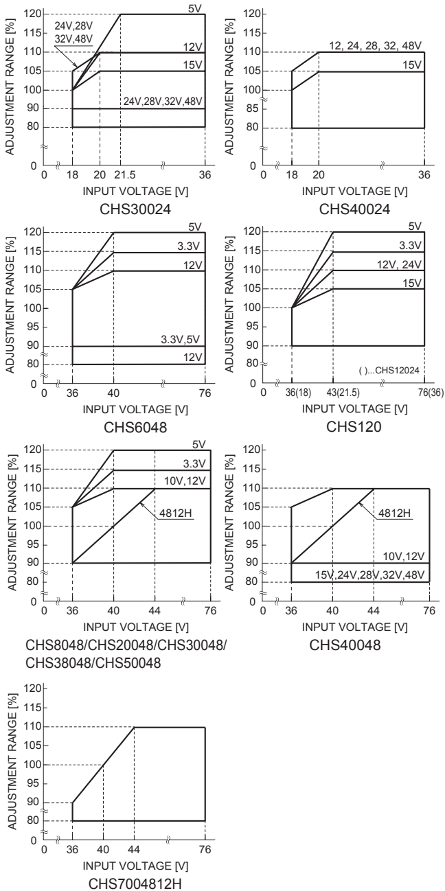
Fig.4.7 CHS Output Voltage Adjustment Range
