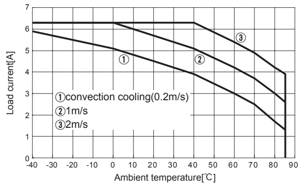
Fig.8.40 Load current vs. ambient temperature(CHS4002448 Vin=24V)
