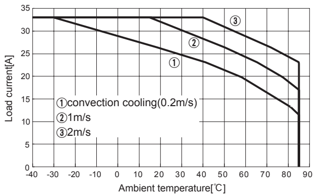
Fig.8.43 Load current vs. ambient temperature(CHS4004812H Vin=48V)
