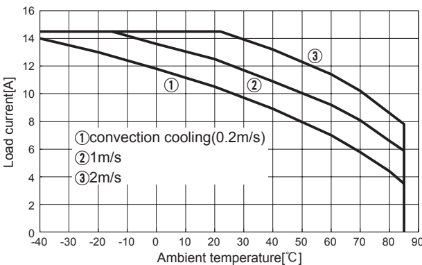
Fig.8.37 Load current vs. ambient temperature(CHS4002424 Vin=24V)
