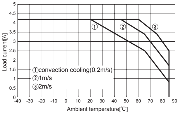
Fig.8.18 Load current vs. ambient temperature(CHS1204824 Vin=48V)
