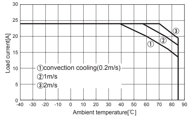
Fig.8.15 Load current vs. ambient temperature(CHS1204805 Vin=48V)
