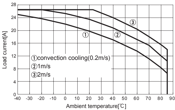
Fig.8.35 Load current vs. ambient temperature(CHS4002412 Vin=24V)
