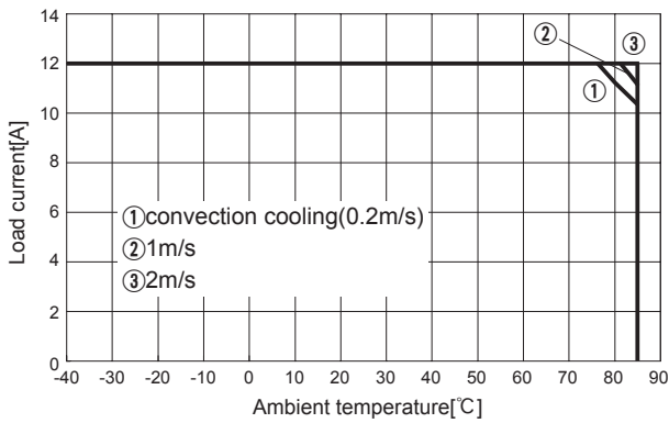
Fig.8.5 Load current vs. ambient temperature(CHS604805 Vin=48V)
