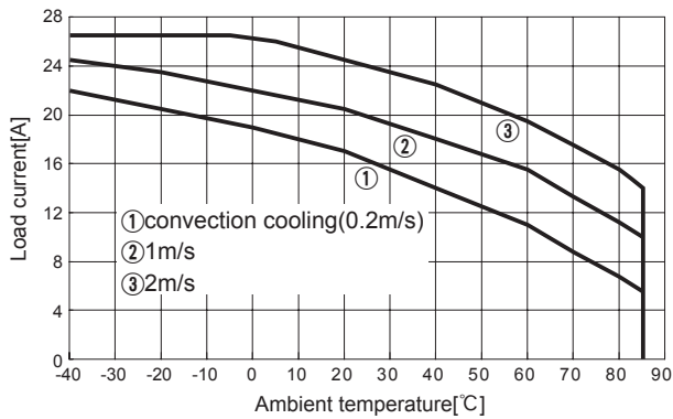
Fig.8.44 Load current vs. ambient temperature(CHS4004815 Vin=48V)
