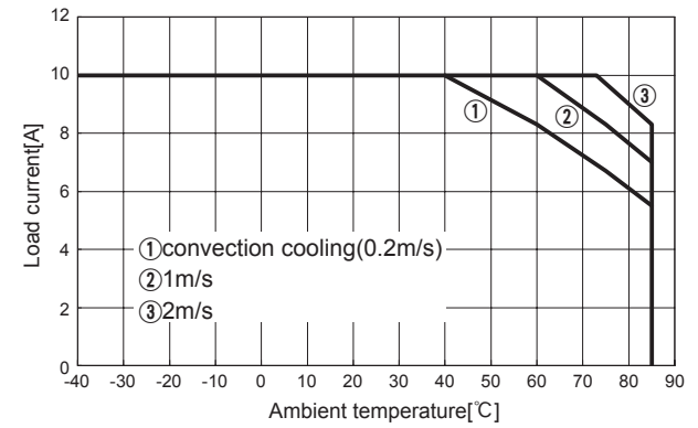
Fig.8.16 Load current vs. ambient temperature(CHS1204812 Vin=48V)
