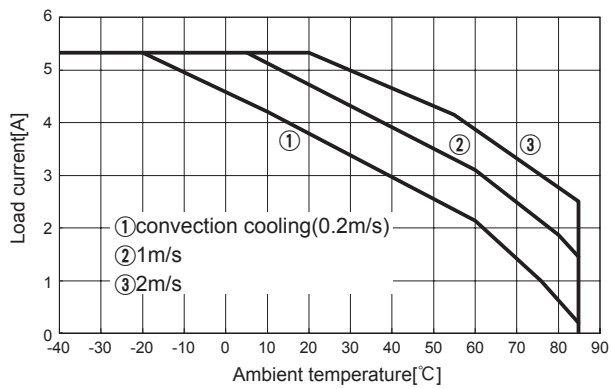
Fig.8.28 Load current vs. ambient temperature(CHS3002448 Vin=24V)
