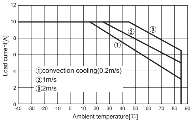
Fig.8.11 Load current vs. ambient temperature(CHS1202412 Vin=24V)
