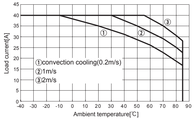
Fig.8.22 Load current vs. ambient temperature(CHS3002405 Vin=24V)
