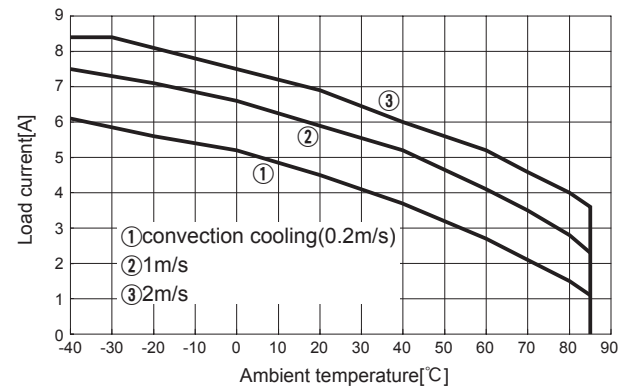
Fig.8.48 Load current vs. ambient temperature(CHS4004848 Vin=48V)
