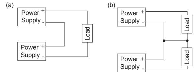
Fig.5.1 Examples of series operation
