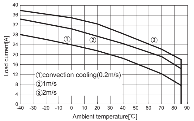
Fig.8.32 Load current vs. ambient temperature(CHS3804810 Vin=48V)
