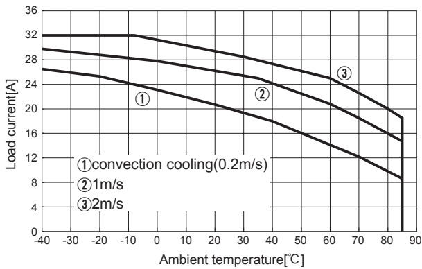
Fig.8.34 Load current vs. ambient temperature(CHS3804812H Vin=48V)
