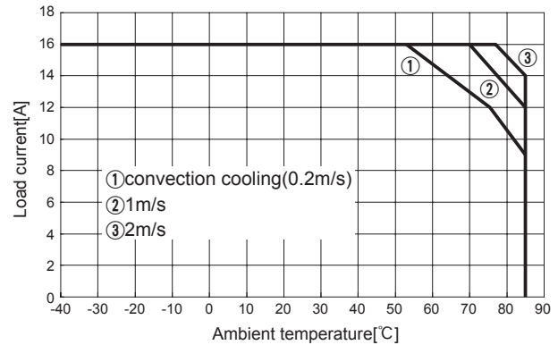
Fig.8.8 Load current vs. ambient temperature(CHS804805 Vin=48V)
