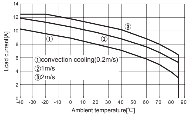
Fig.8.38 Load current vs. ambient temperature(CHS4002428 Vin=24V)
