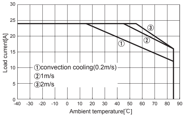
Fig.8.10 Load current vs. ambient temperature(CHS1202405 Vin=24V)
