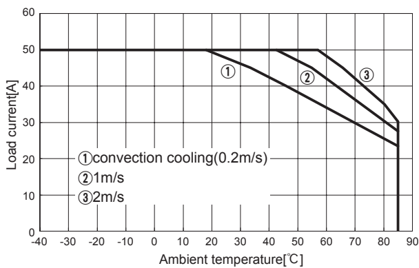
Fig.8.19 Load current vs. ambient temperature(CHS200483R3 Vin=48V)
