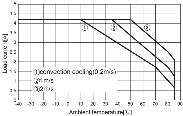
Fig.8.13 Load current vs. ambient temperature(CHS1202424 Vin=24V)
