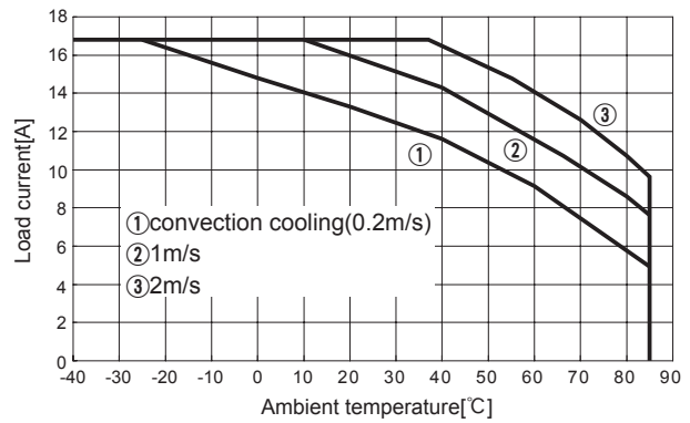
Fig.8.23 Load current vs. ambient temperature(CHS3002412 Vin=24V)
