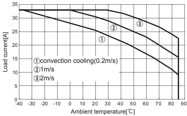
Fig.8.42 Load current vs. ambient temperature(CHS4004812 Vin=48V)
