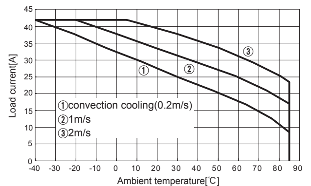
Fig.8.49 Load current vs. ambient temperature(CHS5004812 Vin=48V)
