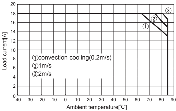
Fig.8.4 Load current vs. ambient temperature(CHS60483R3 Vin=48V)
