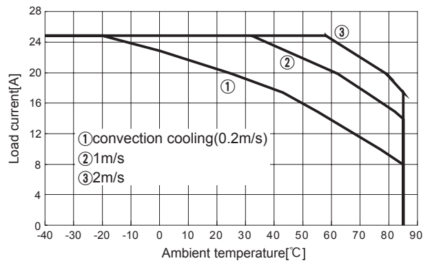
Fig.8.31 Load current vs. ambient temperature(CHS3004812H Vin=48V)
