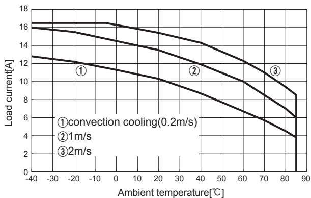
Fig.8.45 Load current vs. ambient temperature(CHS4004824 Vin=48V)
