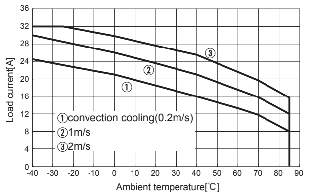
Fig.8.33 Load current vs. ambient temperature(CHS3804812 Vin=48V)
