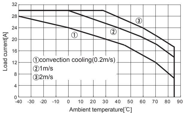
Fig.8.29 Load current vs. ambient temperature(CHS3004810 Vin=48V)
