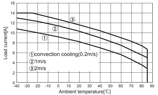
Fig.8.46 Load current vs. ambient temperature(CHS4004828 Vin=48V)
