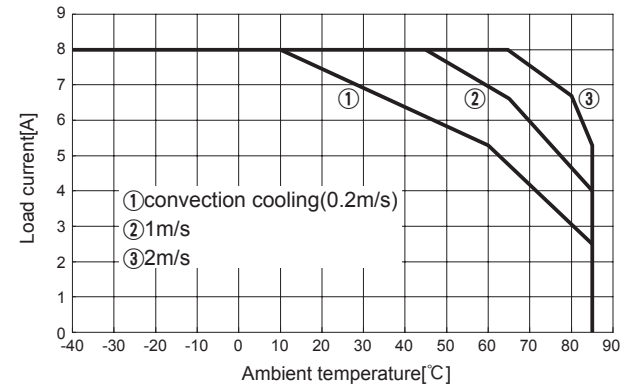
Fig.8.17 Load current vs. ambient temperature(CHS1204815 Vin=48V)
