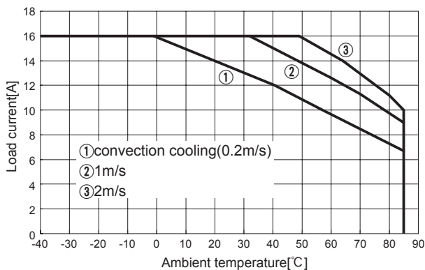
Fig.8.21 Load current vs. ambient temperature(CHS2004812 Vin=48V)
