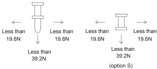
Fig.6.4 Stress to the pins
