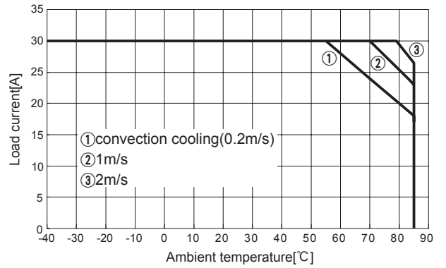
Fig.8.14 Load current vs. ambient temperature(CHS120483R3 Vin=48V)
