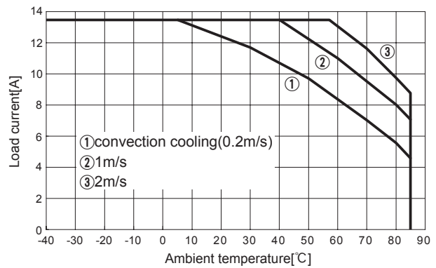
Fig.8.24 Load current vs. ambient temperature(CHS3002415 Vin=24V)
