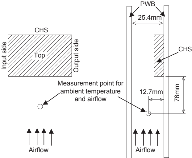
Fig.8.3 Measuring method
