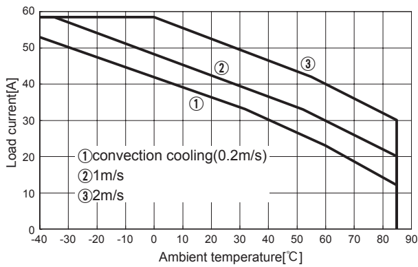
Fig.8.50 Load current vs. ambient temperature(CHS7004812H Vin=48V)
