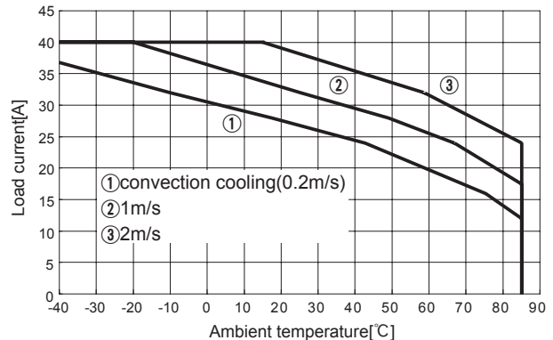
Fig.8.41 Load current vs. ambient temperature(CHS4004810 Vin=48V)
