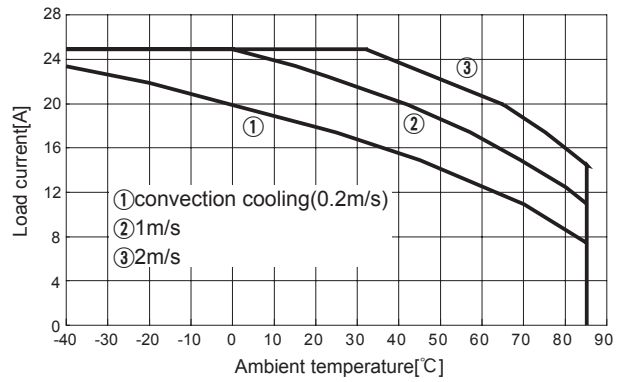
Fig.8.30 Load current vs. ambient temperature(CHS3004812 Vin=48V)
