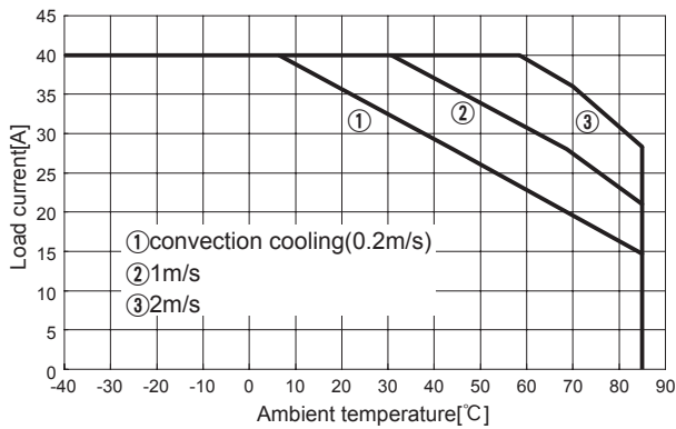
Fig.8.20 Load current vs. ambient temperature(CHS2004805 Vin=48V)
