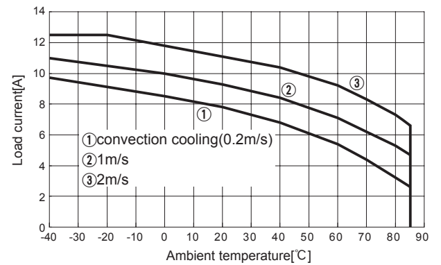
Fig.8.47 Load current vs. ambient temperature(CHS4004832 Vin=48V)
