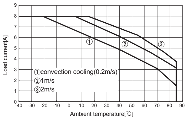
Fig.8.27 Load current vs. ambient temperature(CHS3002432 Vin=24V)
