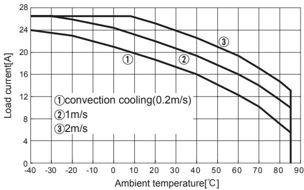
Fig.8.36 Load current vs. ambient temperature(CHS4002415 Vin=24V)
