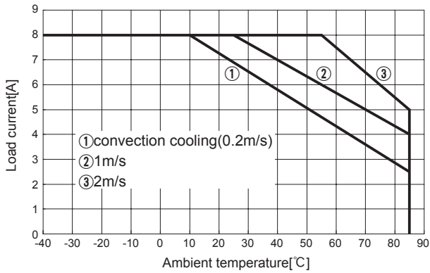
Fig.8.12 Load current vs. ambient temperature(CHS1202415 Vin=24V)
