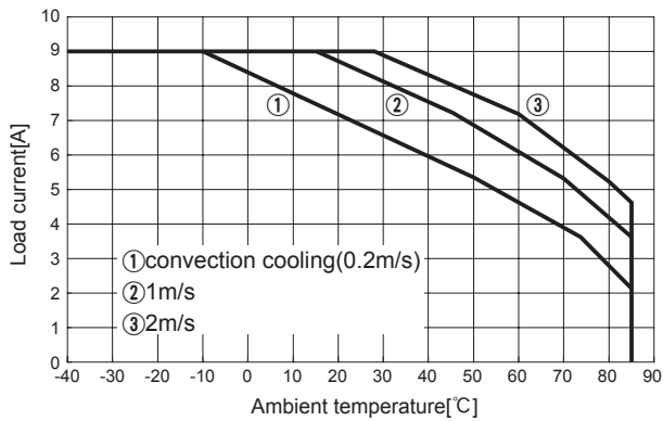
Fig.8.26 Load current vs. ambient temperature(CHS3002428 Vin=24V)
