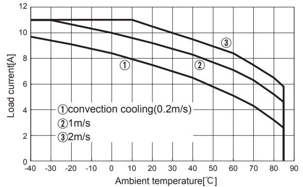
Fig.8.39 Load current vs. ambient temperature(CHS4002432 Vin=24V)
