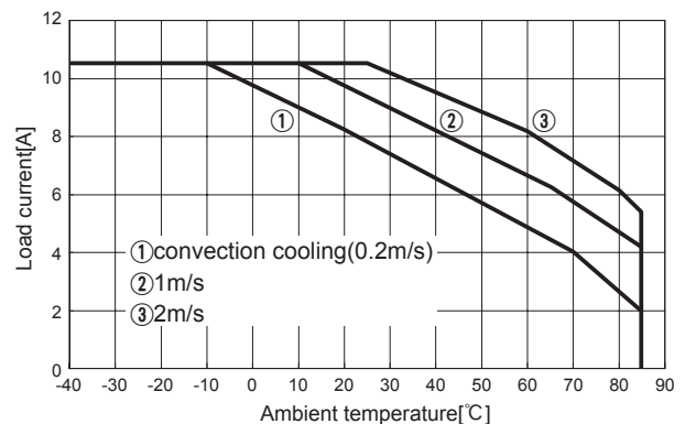
Fig.8.25 Load current vs. ambient temperature(CHS3002424 Vin=24V)
