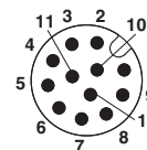
M12 plug connection pin, 12-pos.
