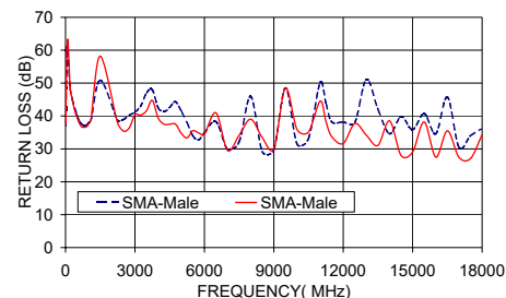
141-3SM+ RETURN LOSS
