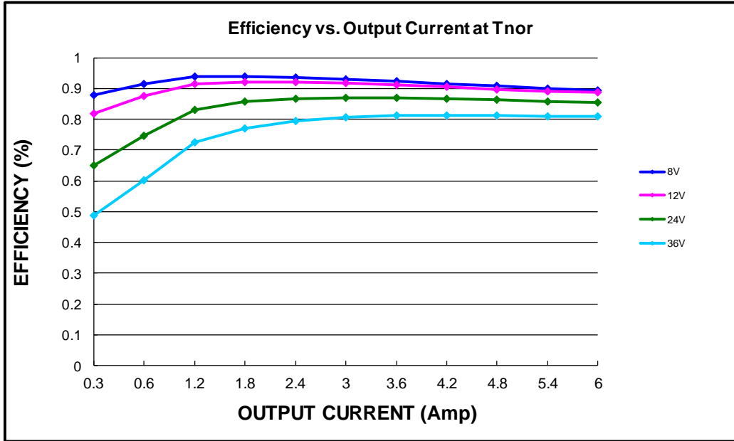
Figure 1. Efficiency data
