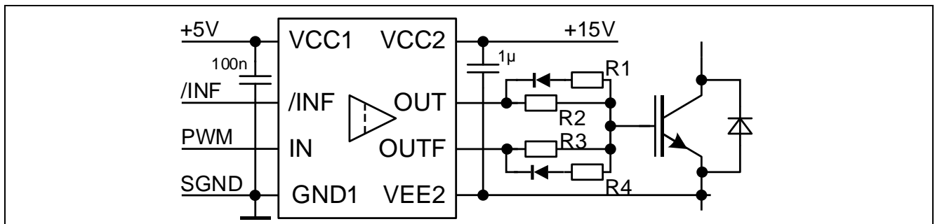
Figure 5 Schematic diagram of the proposed dual-gate resistor gate-drive circuit using 1ED3240MC12H
