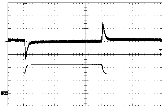
Figure 9. Load Transient Response (100mV/div), di/dt=0.1A/uS, 50% - 75% - 50% of full load, time scale: 200uS/div. Ch2=2A/div
