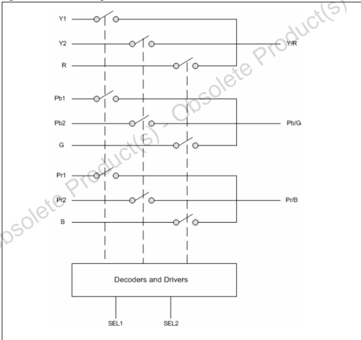
Figure 1. Functional Diagram
