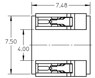
WITH PICK-AND-PLACE CAP
