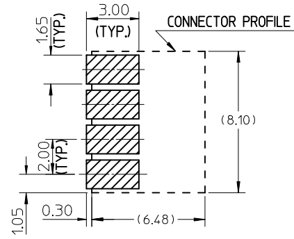
RECOMMENDED FOOT PRINT
