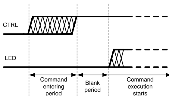
Figure 8. Single-Wire Interface
