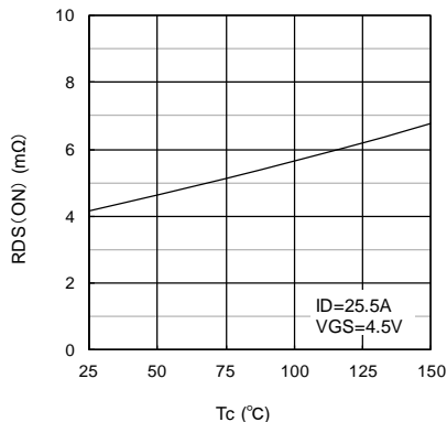
RDS(ON)-Tc characteristics (typical) ID=25.5A, VGS=4.5V
