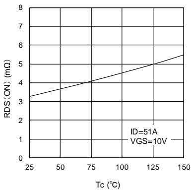
RDS(ON)-Tc characteristics (typical) ID=51A, VGS=10V
