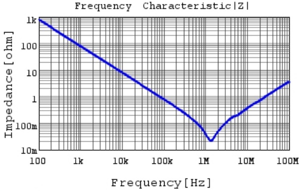
RDED72E225MUE1H03A |Z| DCOV,25degC
