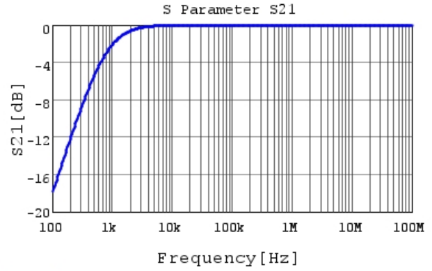
RDED72E225MUE1H03A S21 DCOV, 25degC
