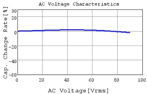
RDED72E225MUE1H03A C-AC Voltage capchange, I
