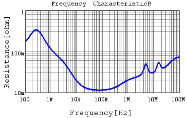
RDED72E225MUE1H03A R DCOV,25degC
