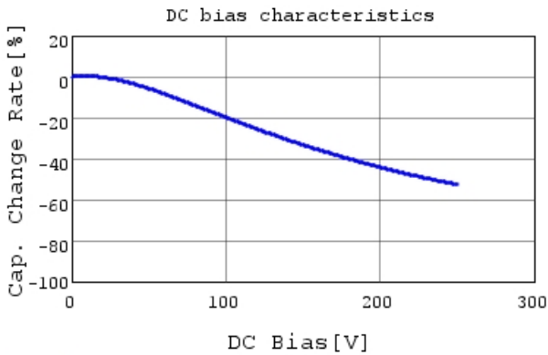
RDED72E225MUE1H03A C-DC bias capchange, 25.0
