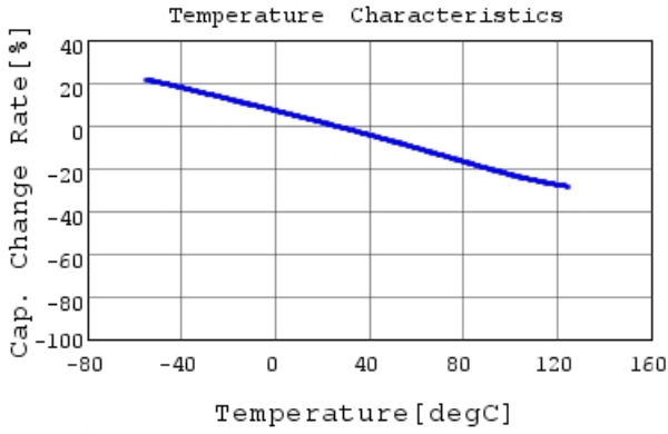
RDED72E225MUE1H03A C-Temp. capchange, DCOV,
