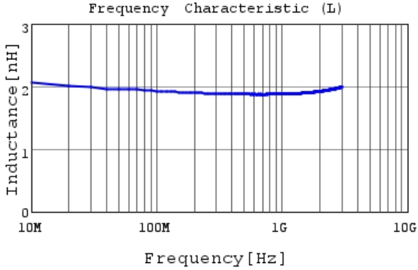
LQG15WZ1N9C02 L
