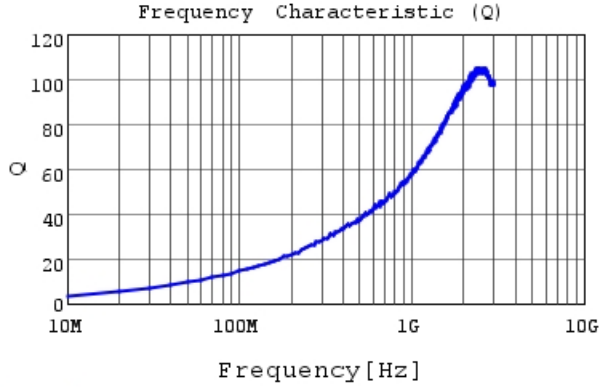
LQG15WZ1N9C02 Q
