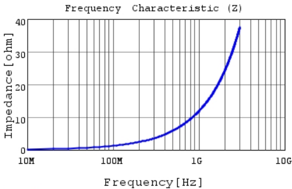
LQG15WZ1N9C02 |Z|
