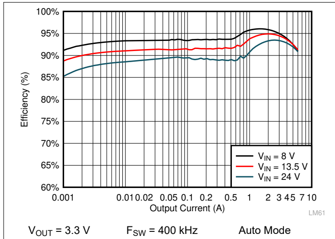
Figure 10-5. LMQ61460-Q1 Efficiency
