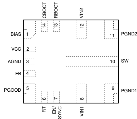
Figure 7-1. RJR Package 14-Pin VQFN-HR Top View
