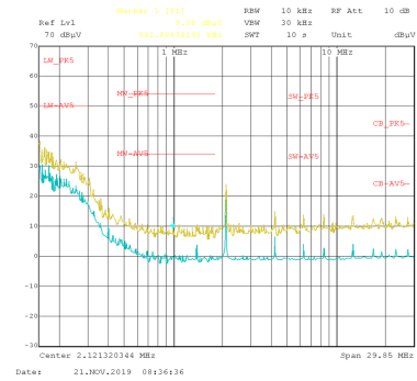
Figure 10-54. Conducted EMI versus CISPR25 Limits (Yellow: Peak Signal, Blue: Average Signal) F SW = 2100 kHz V OUT = 5 V I OUT = 5 A Frequency Tested: 150 kHz to 30 MHz
