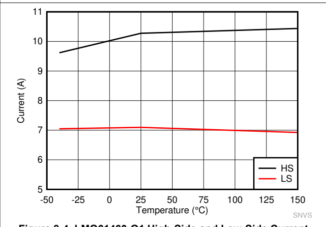
Figure 8-4. LMQ61460-Q1 High-Side and Low-Side Current Limits
