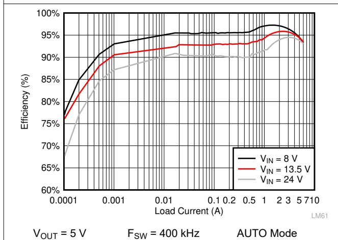
Figure 10-9. LMQ61460-Q1 Efficiency
