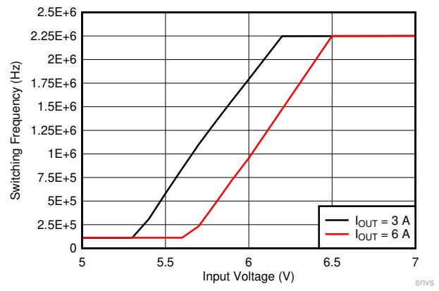
Figure 10-26. LMQ61460-Q1 Frequency Dropout Curve
