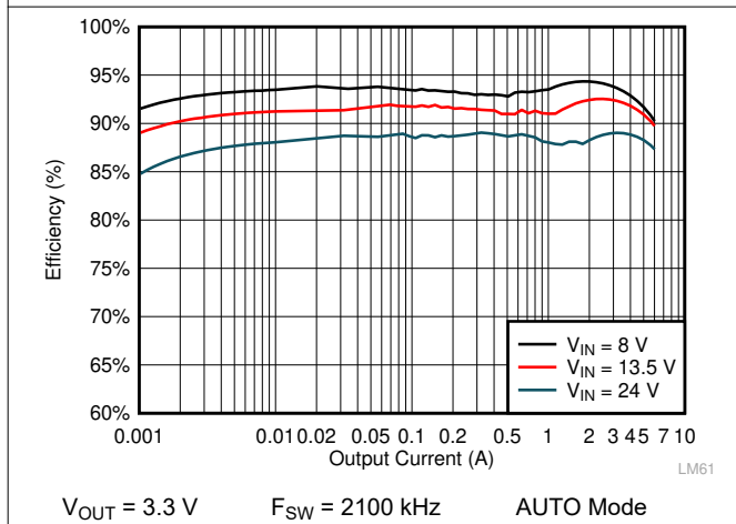
Figure 10-7. LMQ61460-Q1 Efficiency
