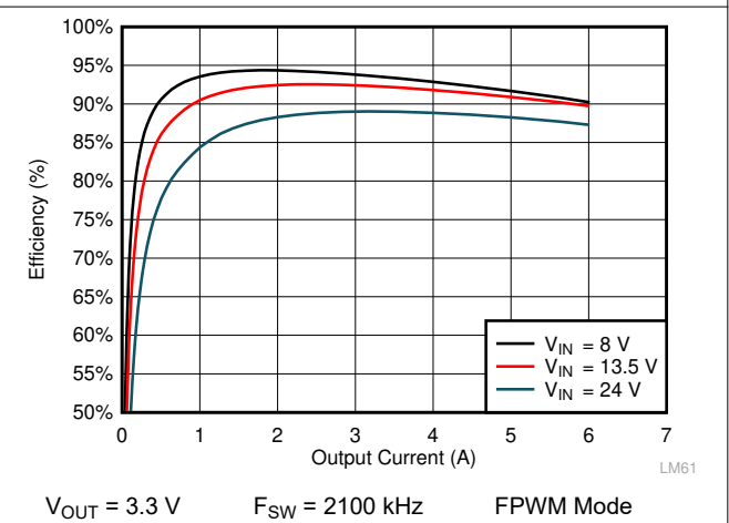
Figure 10-8. LMQ61460-Q1 Efficiency
