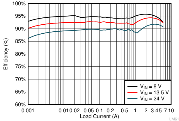
Figure 10-11. LMQ61460-Q1 Efficiency
