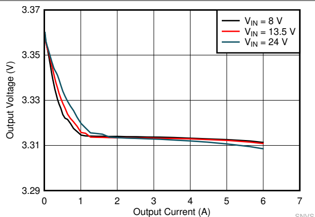
Figure 10-13. LMQ61460-Q1 Load and Line Regulation
