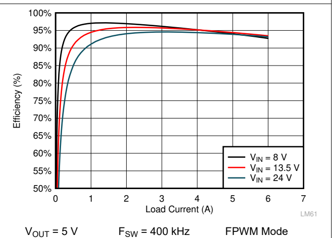
Figure 10-10. LMQ61460-Q1 Efficiency
