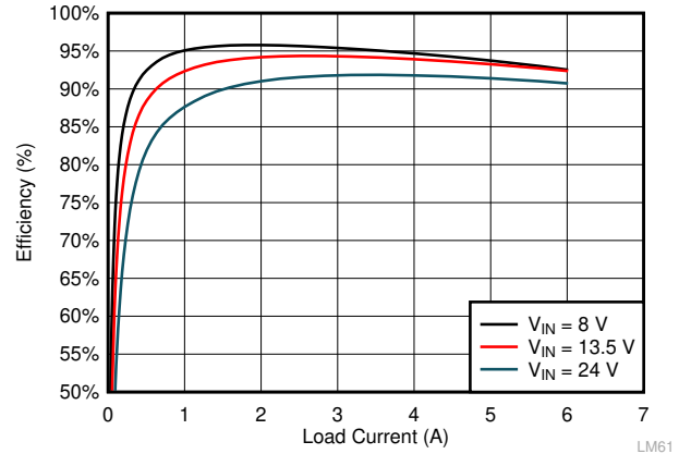
Figure 10-12. LMQ61460-Q1 Efficiency
