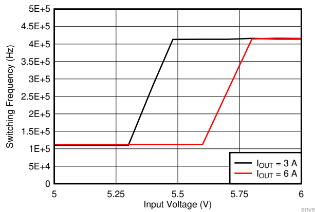
Figure 10-25. LMQ61460-Q1 Frequency Dropout Curve
