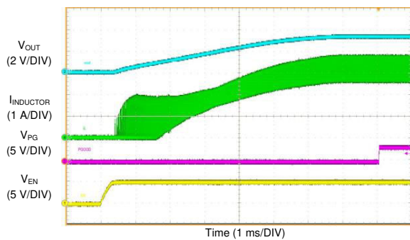
Figure 10-31. LMQ61460-Q1 Start-up with 50-mA Load
