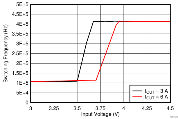
Figure 10-23. LMQ61460-Q1 Dropout Curve
