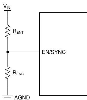
Figure 9-1. V_{IN} SYNC Using the EN pin
