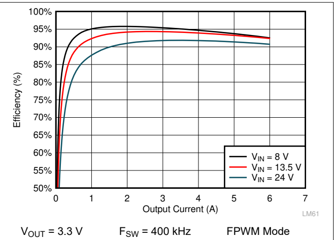
Figure 10-6. LMQ61460-Q1 Efficiency
