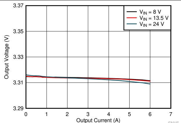
Figure 10-14. LMQ61460-Q1 Load and Line Regulation
