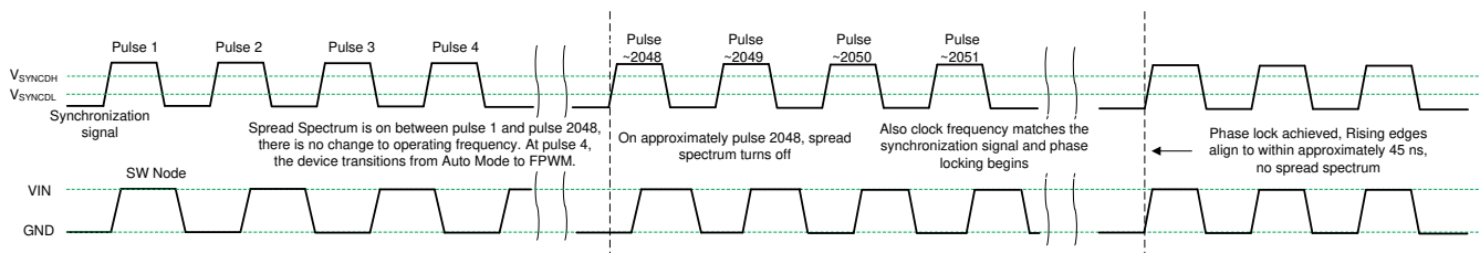
Figure 9-5. Synchronization Process
