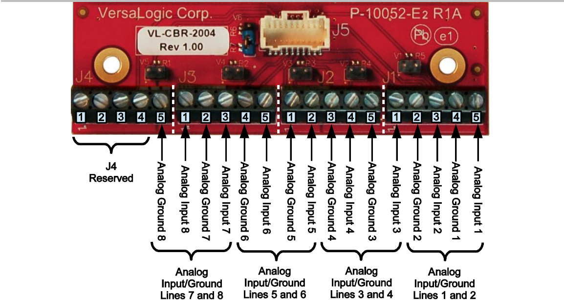
Figure 29. Analog I/O and Ground Terminal Block Pinouts
