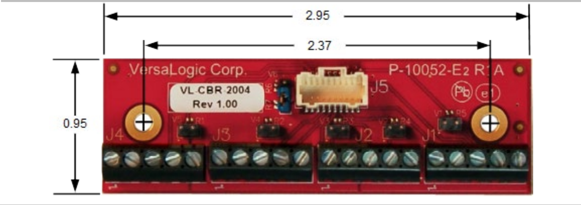
Figure 30. CBR-2004B/CBR-2005 Dimensions and Mounting Holes
