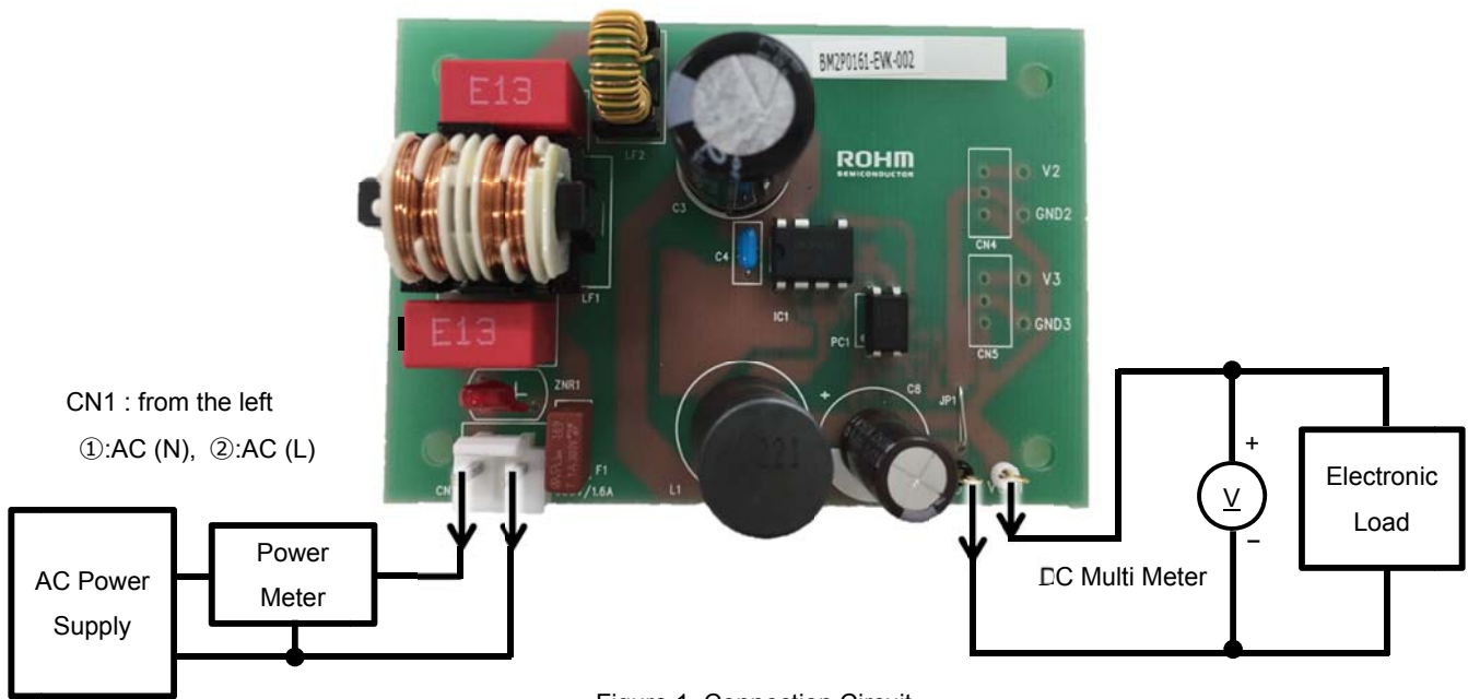
Figure 1. Connection Circuit
