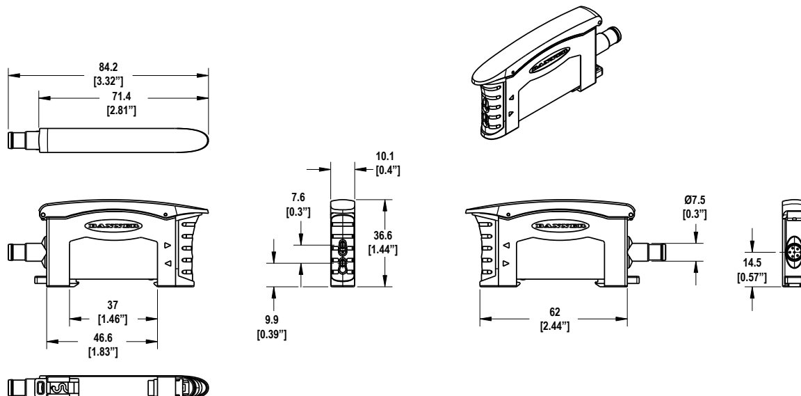
Figure 7. D10 dimensions
