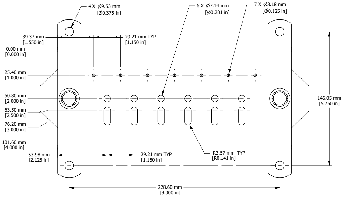
ASSEMBLY - TOP VIEW
