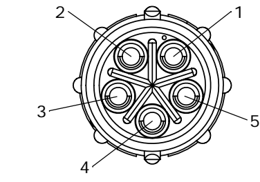
WIRE VIEW 8382-5PG-3XX
