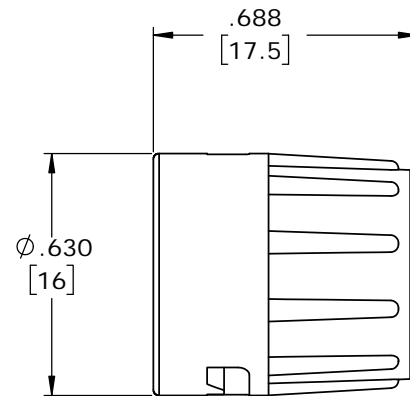
SINGLE GROMMET 8382-XPG-311 .125 I.D. FOR CABLE .09-.14 O.D. [2.3-3.6] 8382-XPG-315 .188 I.D. FOR CABLE .15-.17 O.D. [3.8-4.3] 8382-XPG-318 .156 I.D. FOR CABLE .18-.20 O.D. [4.6-5.1] 8382-XPG-321 .225 I.D. FOR CABLE .21-.23 O.D. [5.3-5.8]
