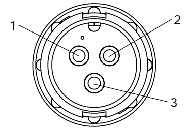
FACE VIEW 8382-3PG-3XX
