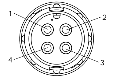
FACE VIEW 8382-4PG-3XX
