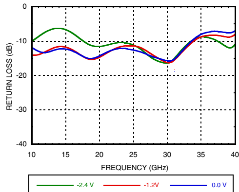
Output Return Loss Vctl1 = 0V, Vctl2 = Variable
