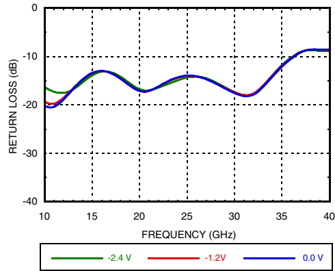
Input Return Loss Vctl1 = 0V, Vctl2 = Variable
