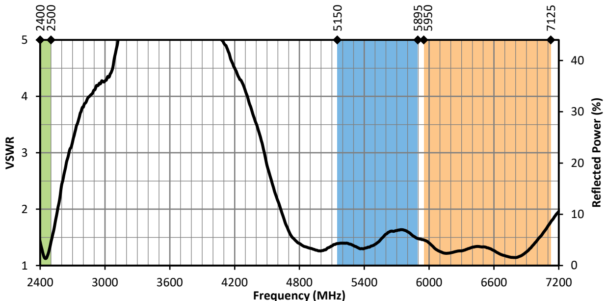
Figure 2. ANT-W63-FPC-SH Antenna VSWR with Frequency Band Highlights
