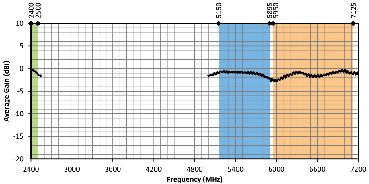
Figure 5. ANT-W63-FPC-SH Antenna Average Gain with Frequency Band Highlights
