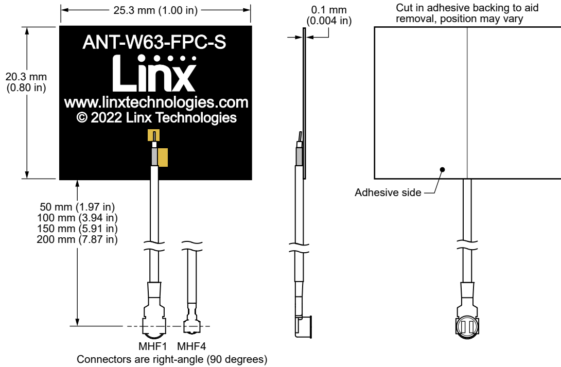
Figure 1. ANT-W63-FPC-SH Series Antenna Dimensions
