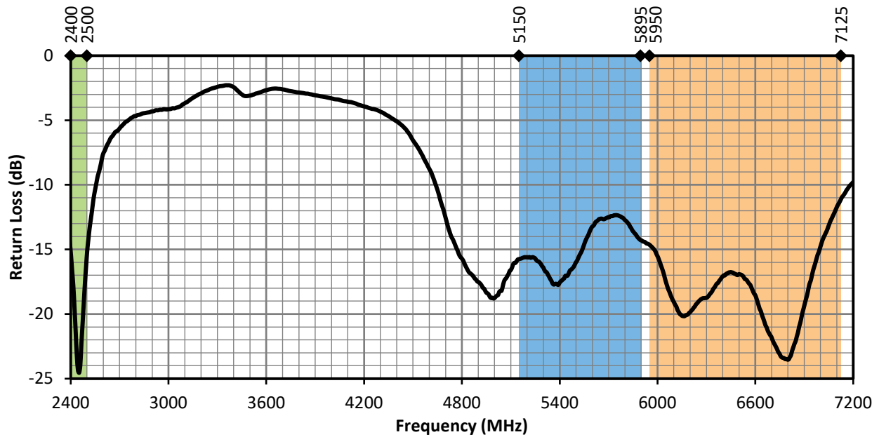
Figure 3. ANT-W63-FPC-SH Antenna Return Loss with Frequency Band Highlights
