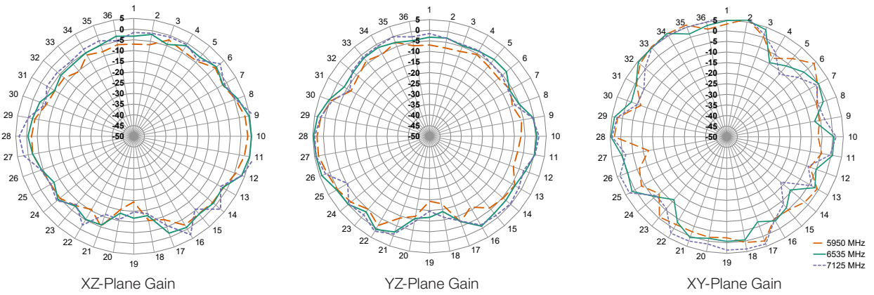
Figure 7. Radiation Patterns for ANT-W63-FPC-SH Series Antenna
