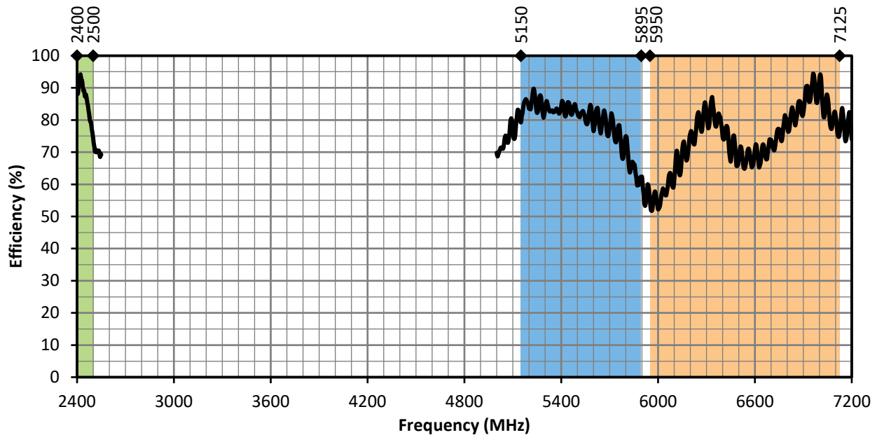
Figure 6. ANT-W63-FPC-SH Antenna Radiation Efficiency with Frequency Band Highlights
