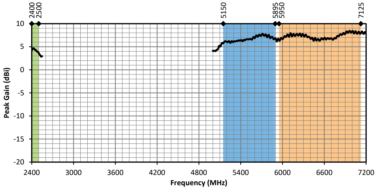
Figure 4. ANT-W63-FPC-SH Antenna Peak Gain with Frequency Band Highlights
