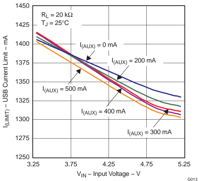
Figure 17. USB Current-Limit Threshold vs V_{IN} , R_{ILIM} = 20\text{ k}\Omega , T_A = 25\text{ }^\circ\text{C}
