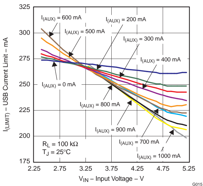
Figure 19. USB Current-Limit Threshold vs V_{IN} , R_{ILIM} = 100\text{ k}\Omega , T_A = 25\text{ }^\circ\text{C}
