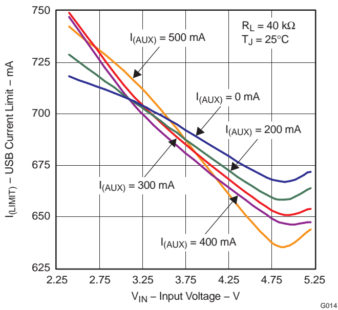
Figure 18. USB Current-Limit Threshold vs V_{IN} , R_{ILIM} = 40\text{ k}\Omega , T_A = 25\text{ }^\circ\text{C}
