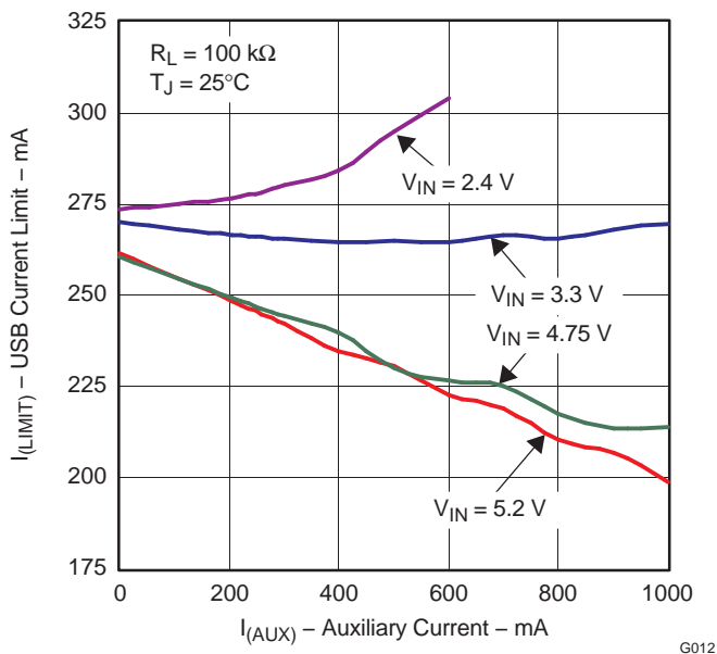
Figure 16. USB Current-Limit Threshold vs I_{AUX} , R_{ILIM} = 100\text{ k}\Omega , T_A = 25\text{ }^\circ\text{C}
