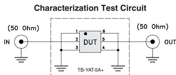
Fig 1. Block diagram of Test Circuit used for characterization, Test board TB-YAT-5A+ Conditions: Attenuation, VSWR: Pin=-10 dBm
