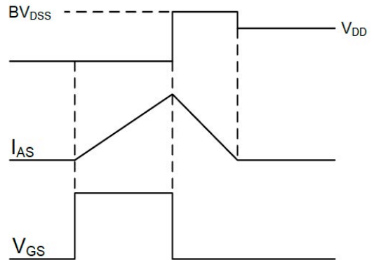
Figure 10. EAS Waveform
