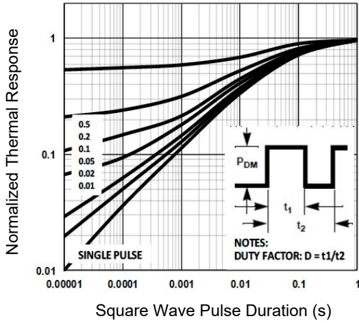
Figure 7. Normalized Transient Impedance
